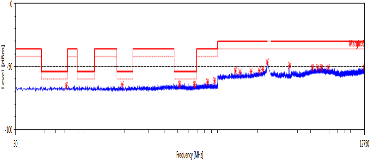
Antenna 1 Tx Spurious Emission
