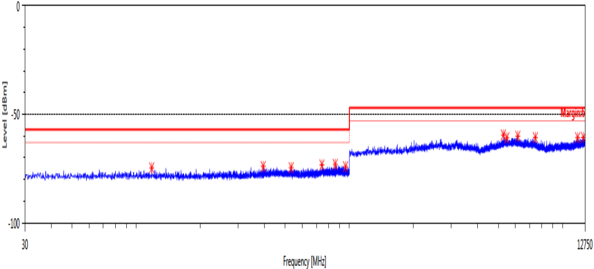
Antenna 1 Rx Spurious Emission
